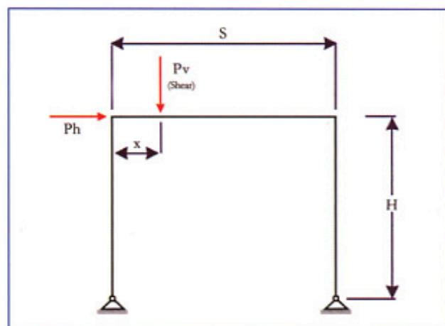
Figure 1 (b): Deck Shear Load
