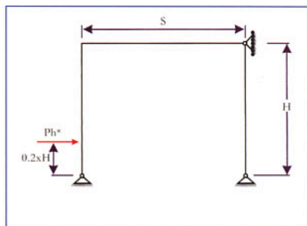
Figure 1 (c): Horizontal Leg Load
